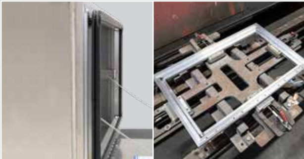
0.125" Aluminum with extruded door frame for maximum strength
